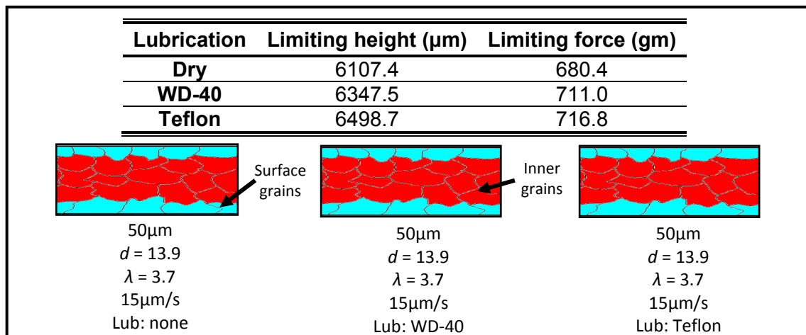
Figure 5- 15 Comparison of limiting values of lubricated 50 \mu\text{m} microformed CuZn30
