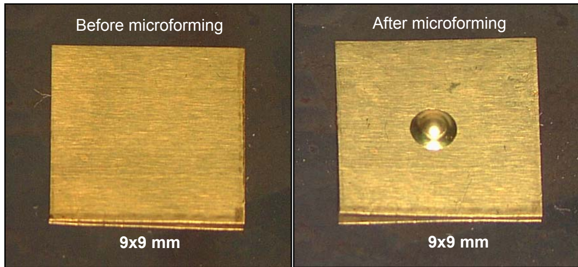
Figure 4- 4 A Test specimen (CuZn30) before and after bulging
