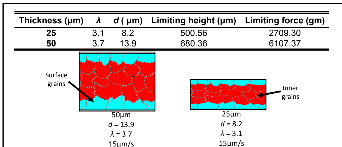
Figure 5- 13 Comparison of limiting values of microformed CuZn30 sheets at 15 \mu\text{m}/\text{s}
